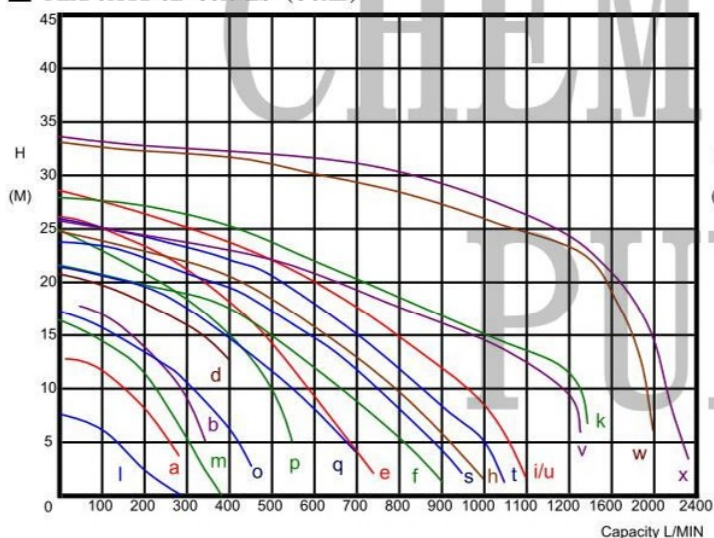
■ PERFORMANCE CURVES (50HZ)
