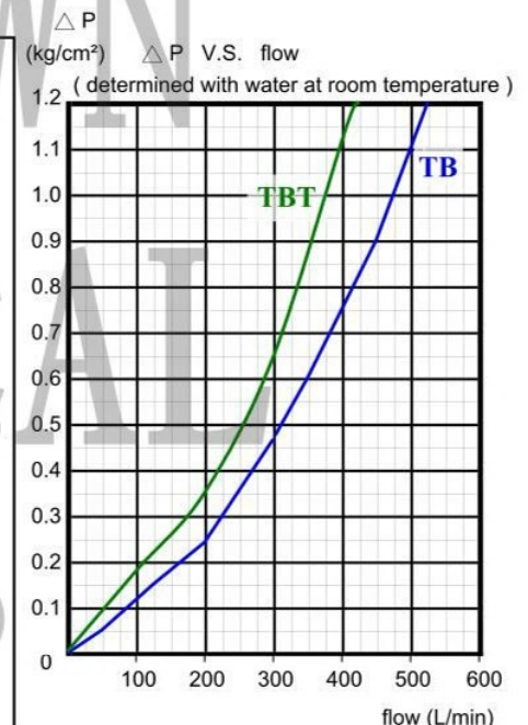
\Delta P : Difference in pressure between inlet & outlet with 50um filter
